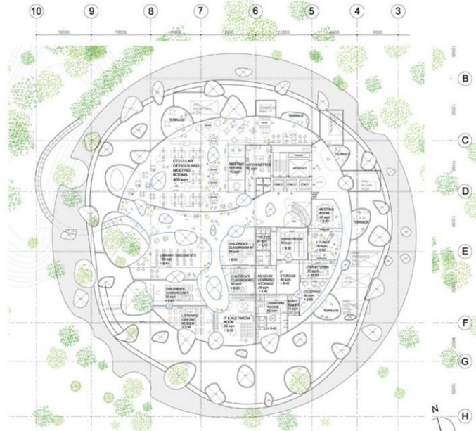
MUSEUM LEARNING & OFFICES First Floor Plan - 1/250
